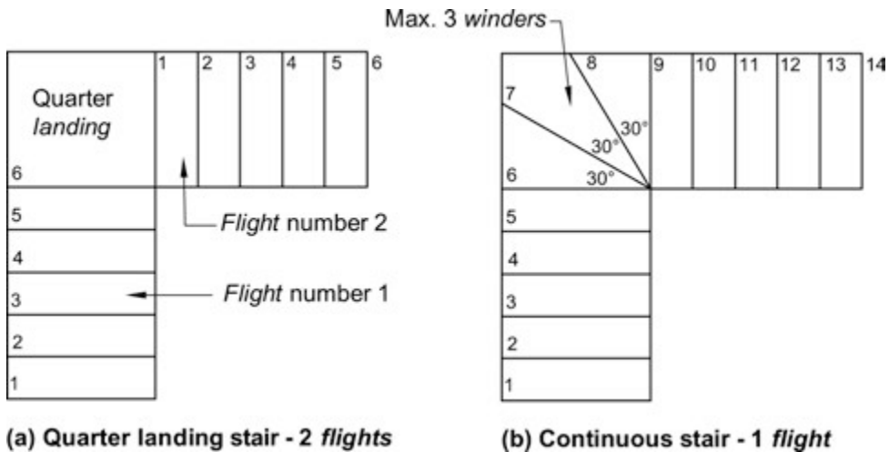
Figure 3.9.1.1 IDENTIFICATION OF STAIR FLIGHTS — Plan view
