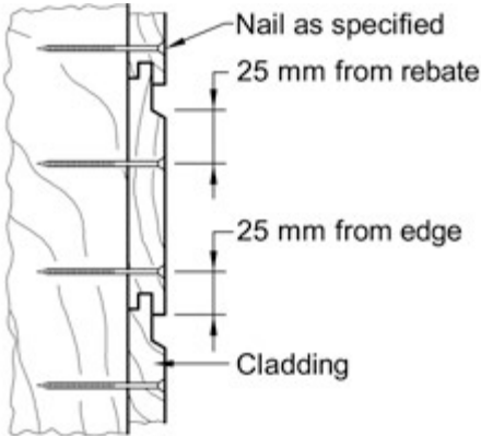
(a) (i) Shiplap weather board
