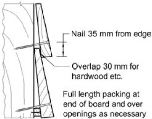
(a) (ii) Splayed weather board
