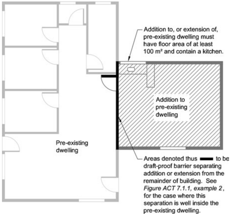
Diagram a. Addition not incorporating floor area from existing dwelling
