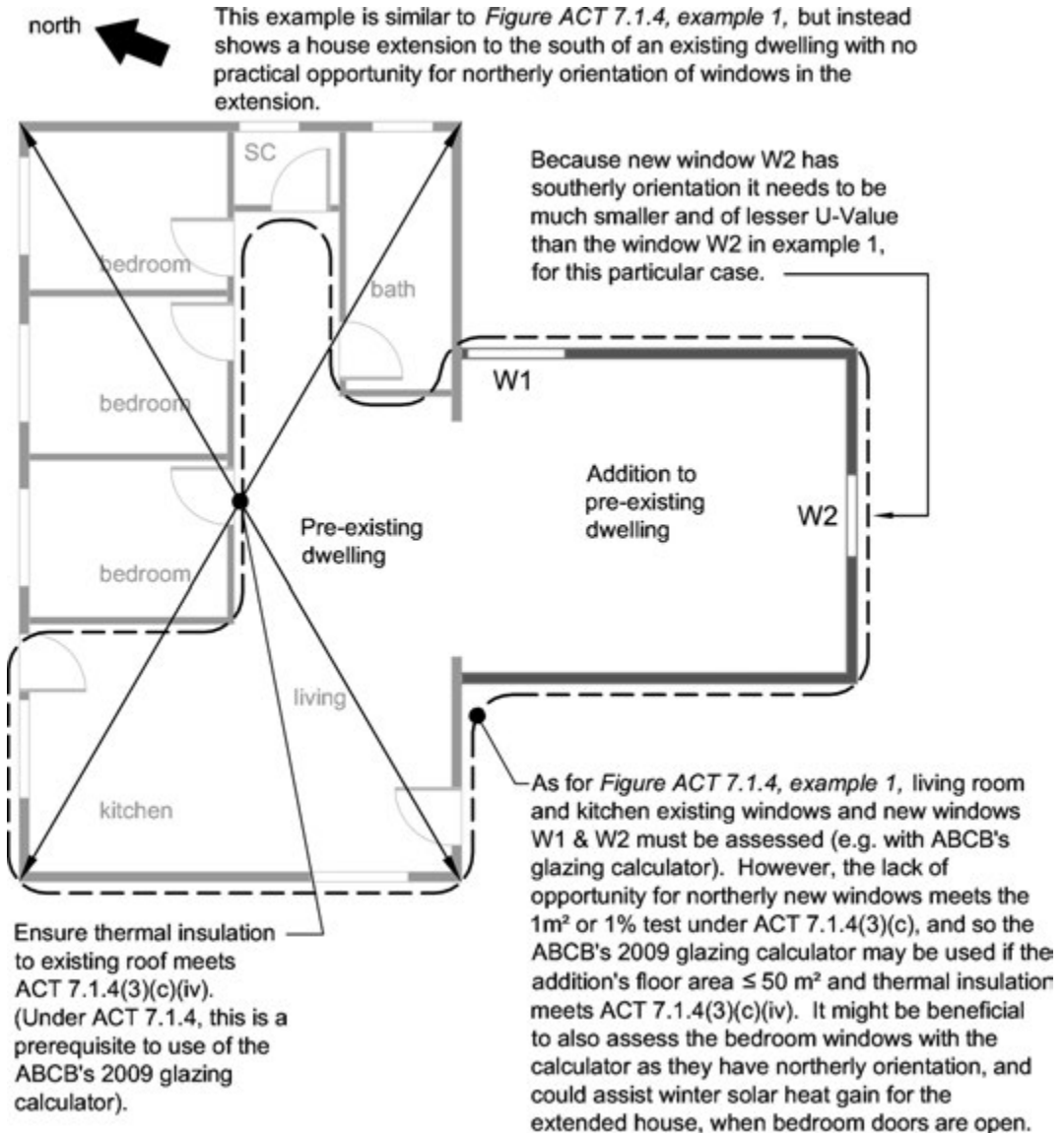
Diagram b. Addition not incorporating a wall within the north sector
